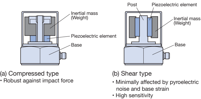
Figure 1: Piezoelectric Accelerometer Structure
