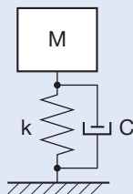
*: A vibration system where M is the mass, k is the spring constant, and C is the viscosity resistance.
